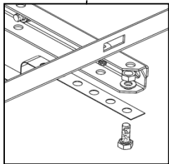
Bolt M10x25 x 2pcs Nut M10 x2pcs Flat washer x2pcs Straps x2pcs
