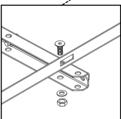
G1030/G2077 x2pcs Bolt sink M10x25 x 2pcs Nut M10 x2pcs Flat washer x2pcs
