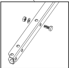
Bolt M10x25 x 2pcs Nut M10 x2pcs Flat washer x2pcs
