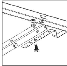
Bolt M10x25 x 2pcs Nut M10 x2pcs Flat washer x2pcs Straps x2pcs
